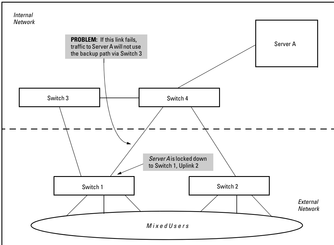
Figure 13-11. Connectivity Problems Using MAC Lockdown with Multiple Paths
